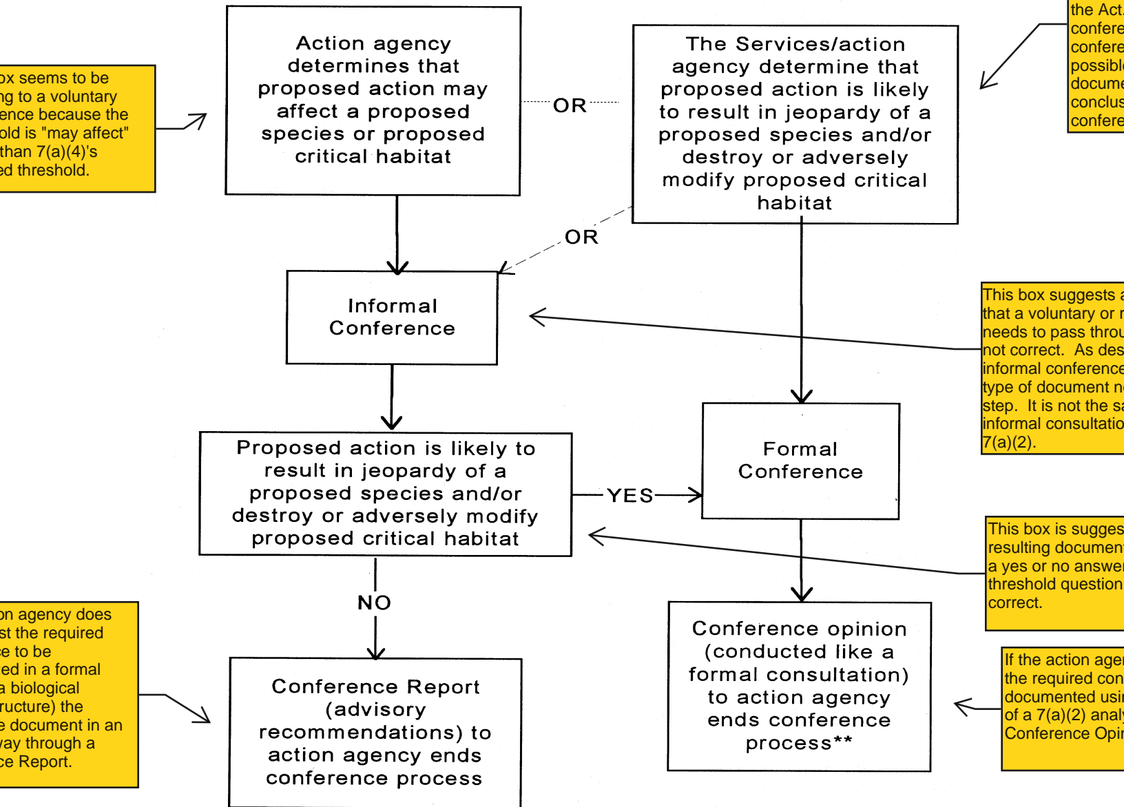
Figure 6-1. Conference processes.
